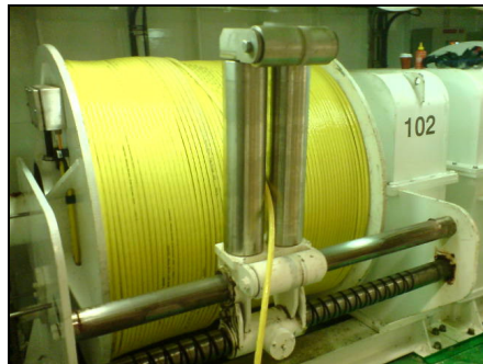
4300 m synthetic rope with fiberoptic cable
