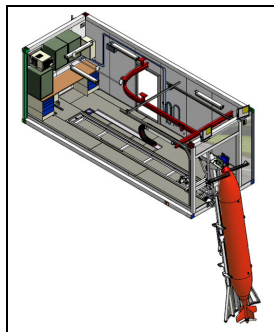
HUGIN AUV
